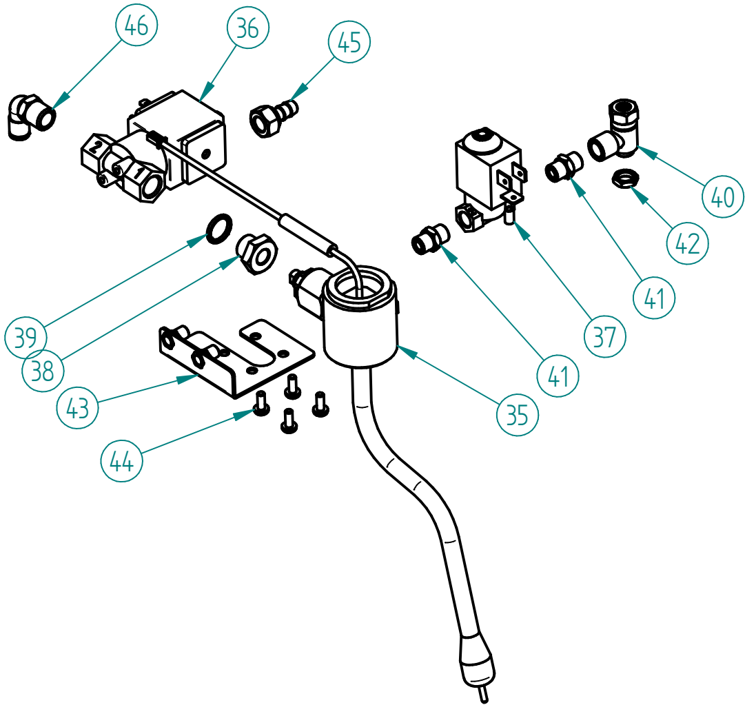
22 - 7.0.007.0123 - TORNEIRA VAPOR C/ Sonda COMPASS 22 - STEAM TAP W/ PROBE COMPASS
