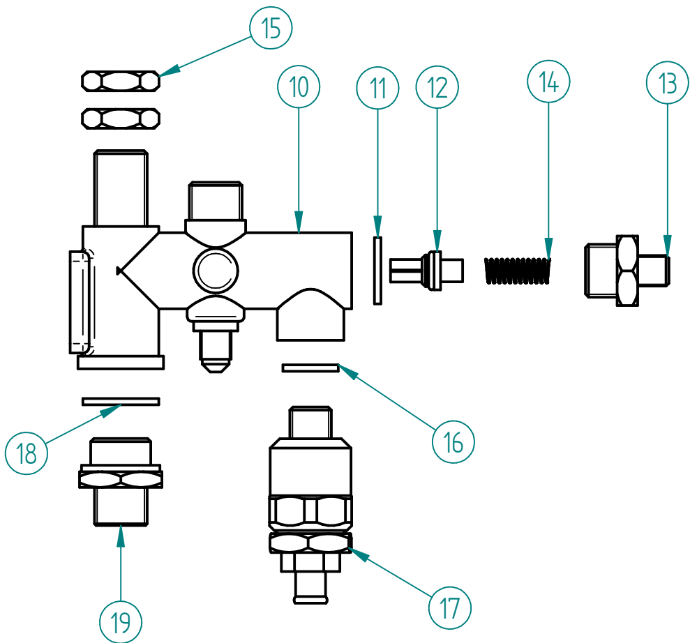
1 – 4.0.016.0010 – BLOCO ENTRADA AGUA ECC-07 (AUT.) 1 – WATER INLET ASS.
