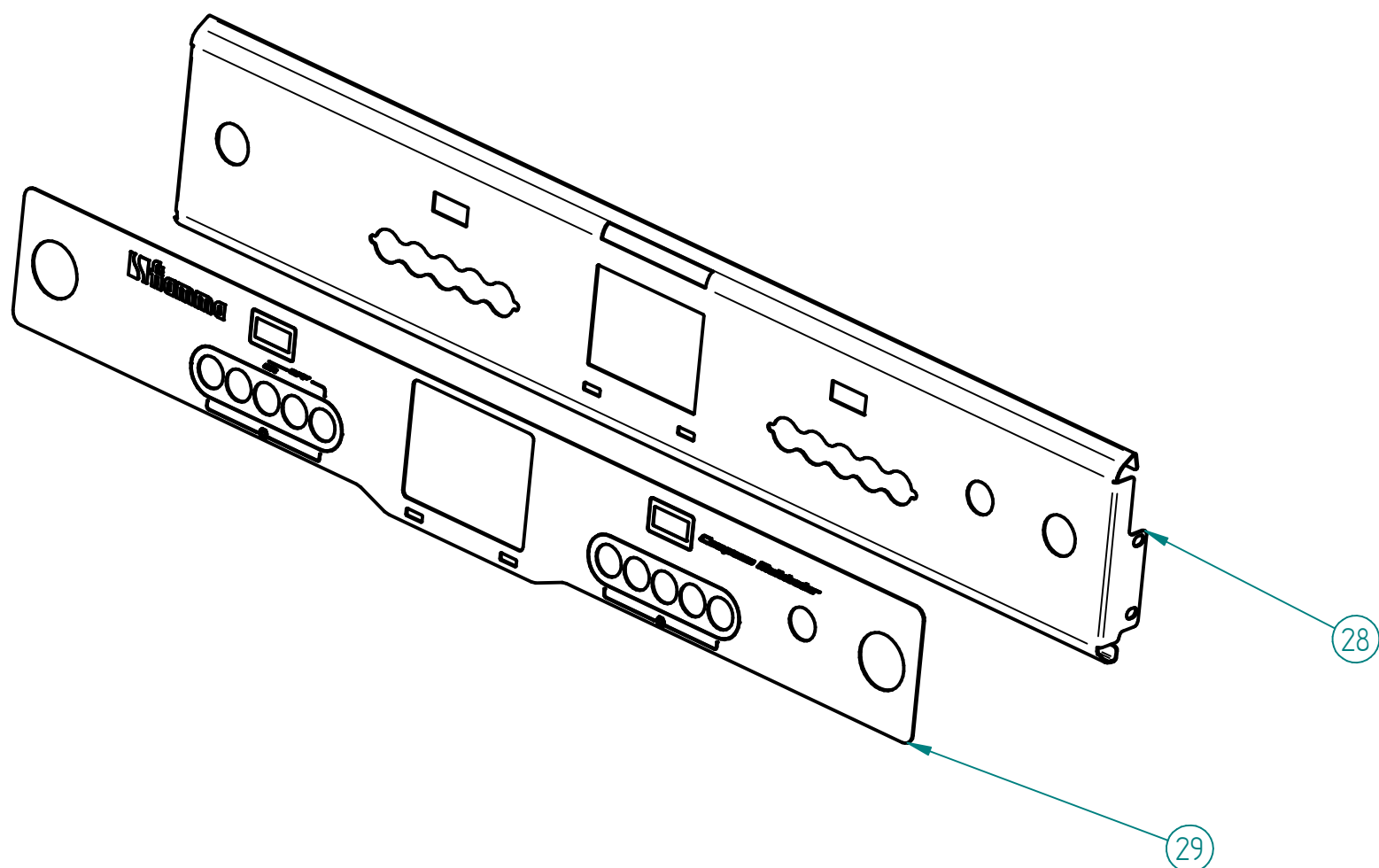
24 - PM_PAINEL COMANDO SUPERIOR CONJ. COMPASS 2 MB TC BLACK 24 - PM_UPPER COMMAND PANEL ASS. COMPASS 2 MB TC BLACK
