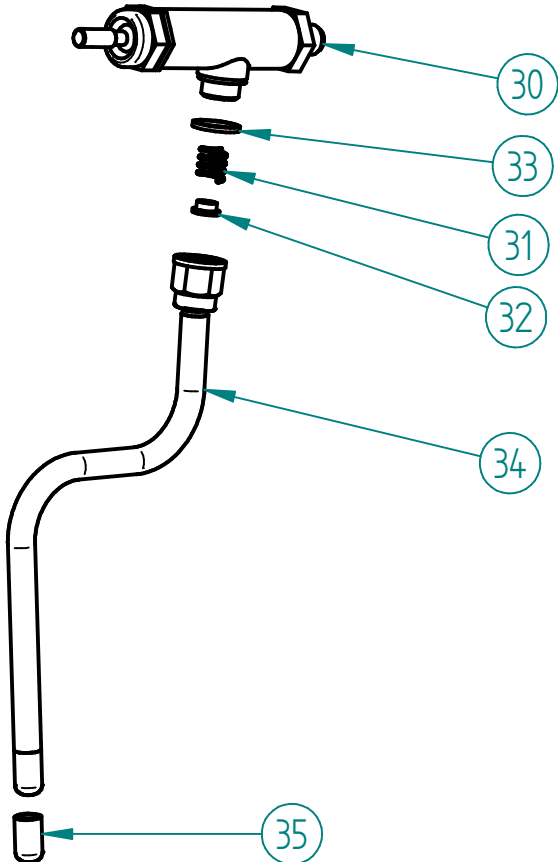
2 – 7.0.007.0150 – TORNEIRA ALAVANCA G1/4-G3/8 RST (CONJ. VAPOR) COOL TOUCH 2 – COOL TOUCH TAP G1/4-G3/8 RST (STEAM ASS.)
