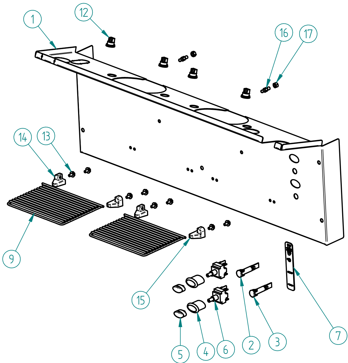
27 - PM_ PAINEL FRONTAL CONJ. COMPASS 2 MB TC 27 - PM_FRONT PANEL COMPASS 2 MB TC
