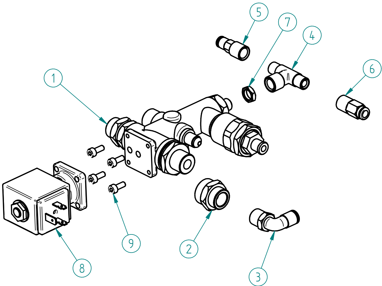
43 – 7.0.028.1150 – BLOCO ENTRADA AGUA ECC-07 CONJ. PACIFIC MB 43 – WATER INLET ASS. PACIFIC MB
