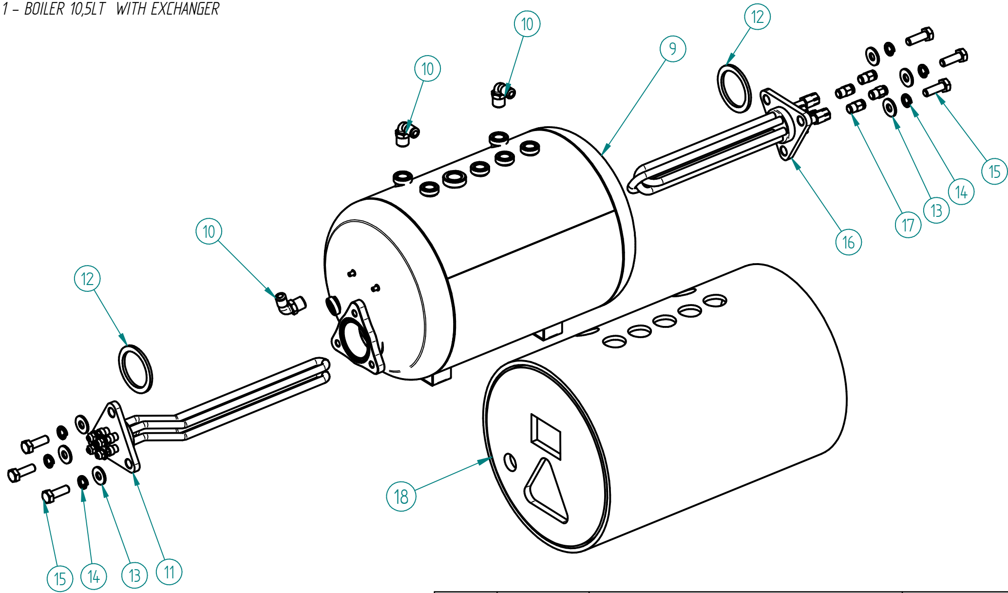
1 - 7.0.000.0552 - CALDEIRA 10,5LT MB C/ PREMUTADOR C/ ACESS. 1 - BOILER 10,5LT WITH EXCHANGER
