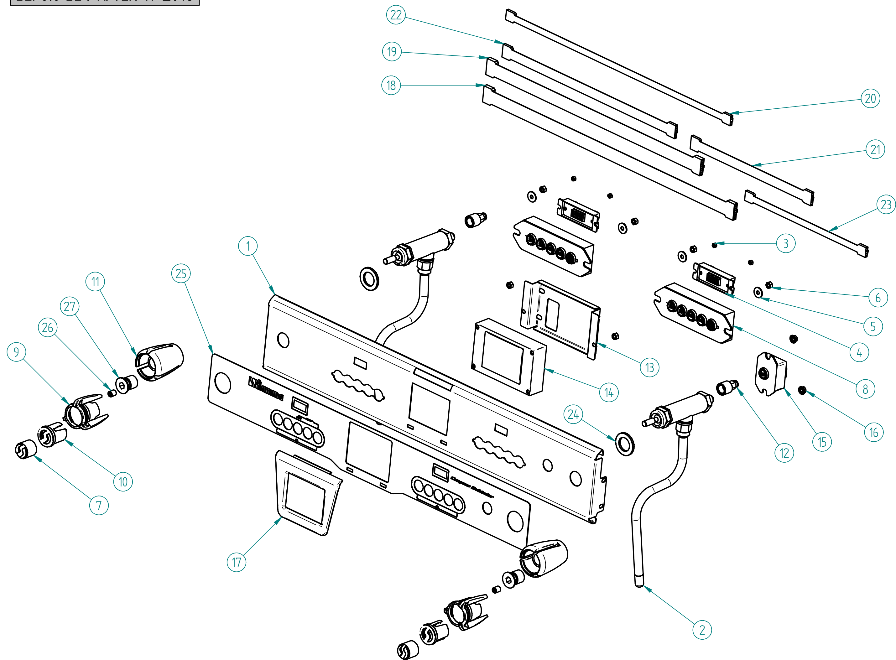
24 - PM_PAINEL COMANDO SUPERIOR CONJ. COMPASS 2 MB TC BLACK 24 - PM_UPPER COMMAND PANEL ASS. COMPASS 2 MB TC BLACK
